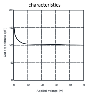
Applied voltage vs. Output capacitance characteristics
