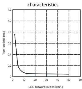
LED forward current vs. Turn on time characteristics
