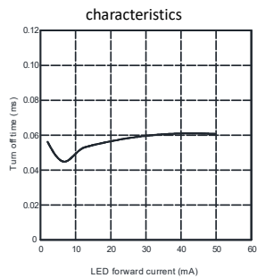
LED forward current vs. Turn off time characteristics
