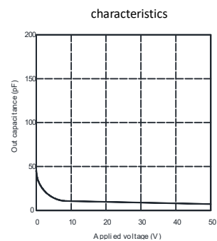
Applied voltage vs. Output capacitance
