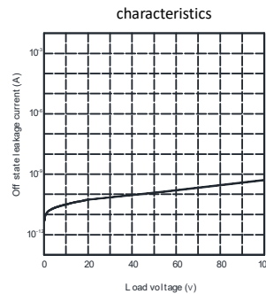
Off state leakage current vs. Load voltage
