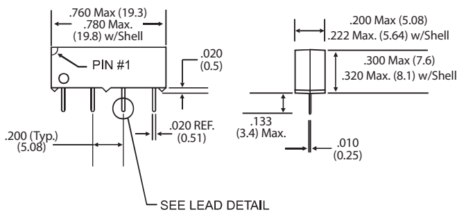
Alternate Package
