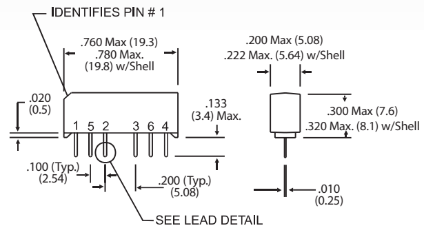
Model 9002
