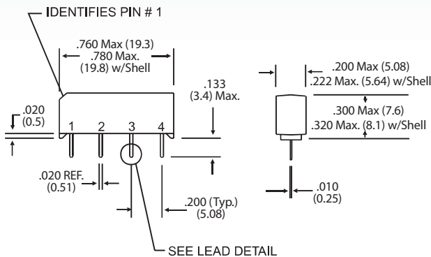
Alternate Package
